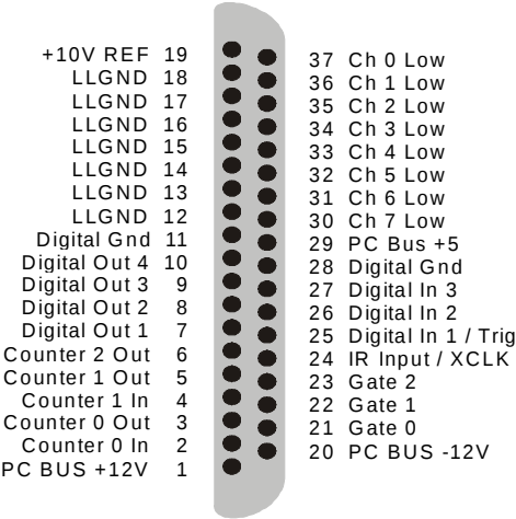
Figure 2-2. BP40-37 Adapter Cable Pinout
