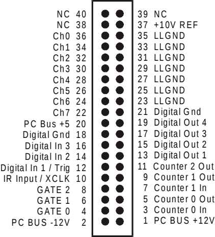
Figure 2-1. Analog Connector
