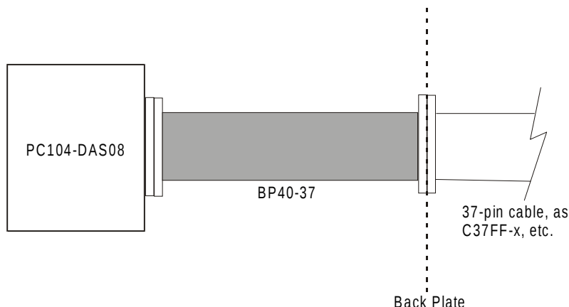
Figure 2-3. BP40-37 Adapter Cabling
